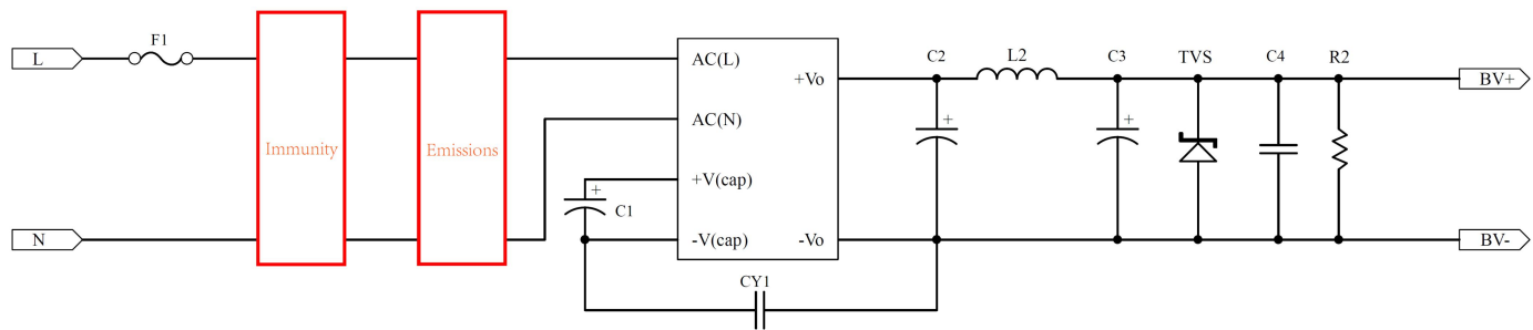
KSE-5W Series additional component selection guide (no EMC devices)
